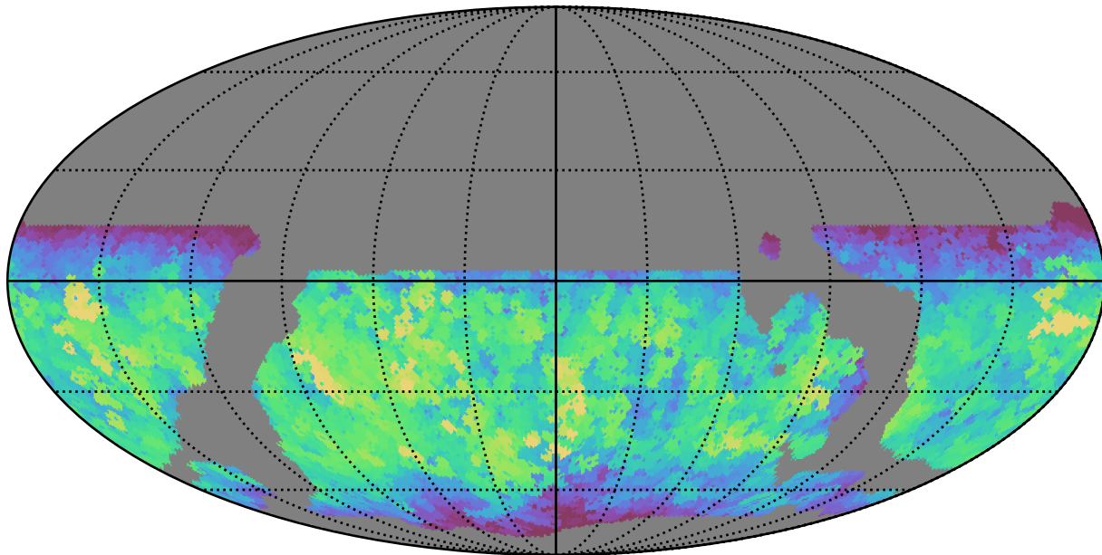
weather_cloudso14v3.4_10yrs WFD y band: Max fiveSigmaDepth
