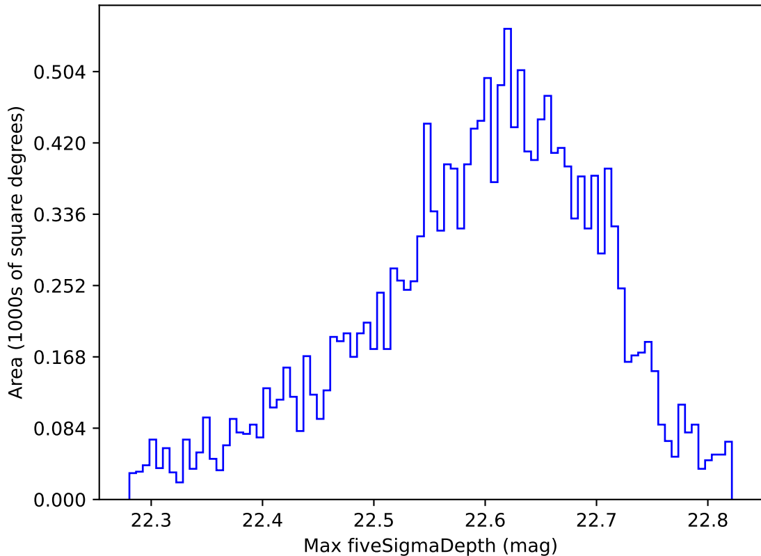
weather_cloudso14v3.4_10yrs WFD y band: Max fiveSigmaDepth
