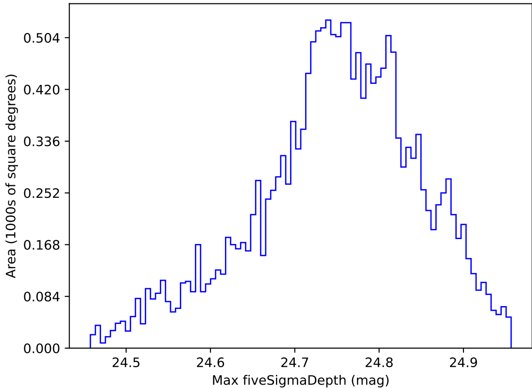
weather_cloudso14v3.4_10yrs WFD r band: Max fiveSigmaDepth
