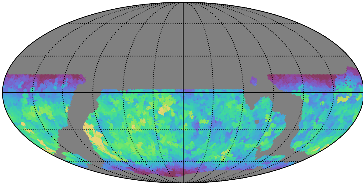
weather_cloudso14v3.4_10yrs WFD i band: Max fiveSigmaDepth
