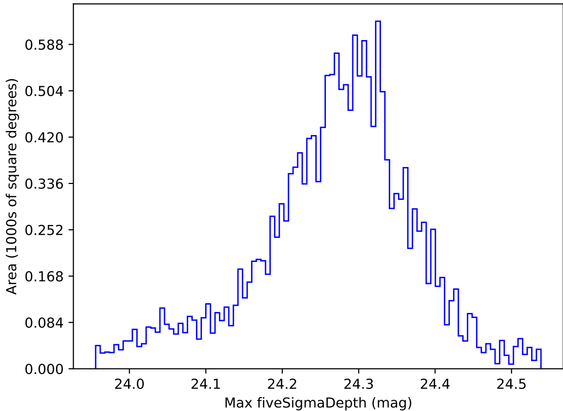
weather_cloudso14v3.4_10yrs WFD i band: Max fiveSigmaDepth
