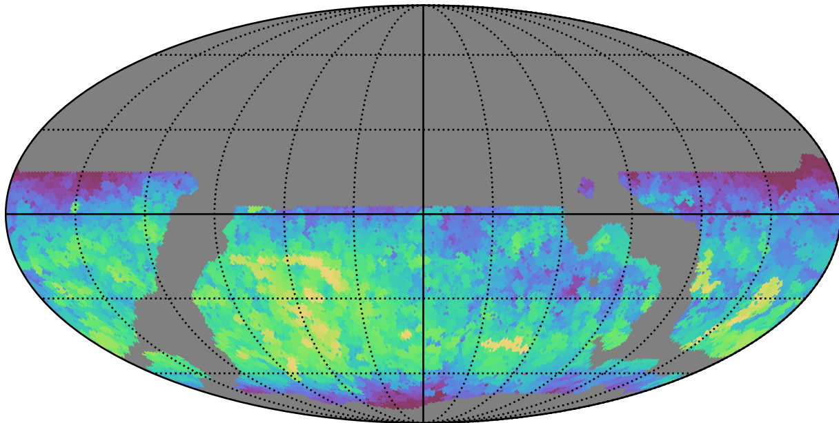
weather_cloudso14v3.4_10yrs WFD g band: Max fiveSigmaDepth
