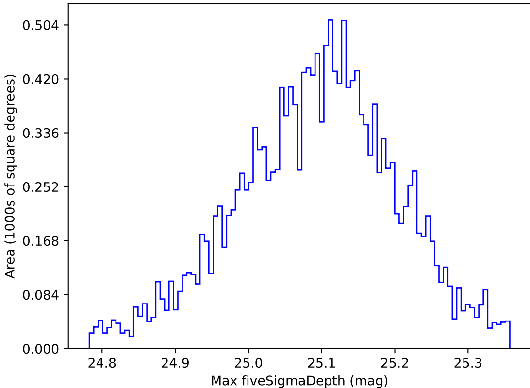
weather_cloudso14v3.4_10yrs WFD g band: Max fiveSigmaDepth
