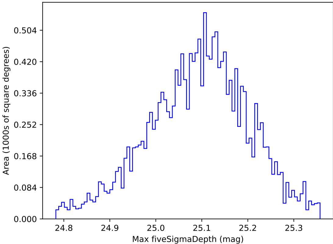
weather_cloudso14v3.4_10yrs WFD all bands: Max fiveSigmaDepth
