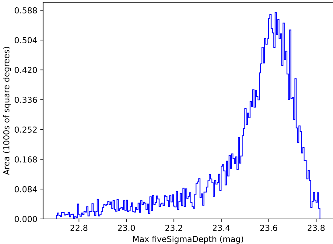
weather_cloudso14v3.4_10yrs All sky z band: Max fiveSigmaDepth
