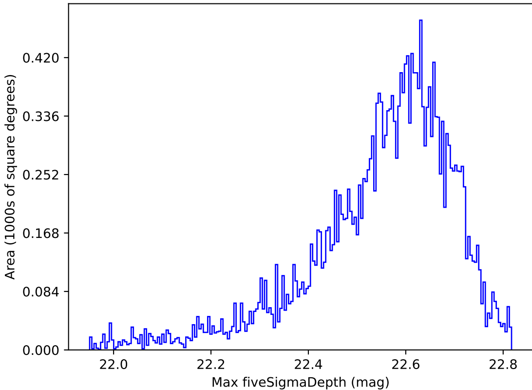
weather_cloudso14v3.4_10yrs All sky y band: Max fiveSigmaDepth
