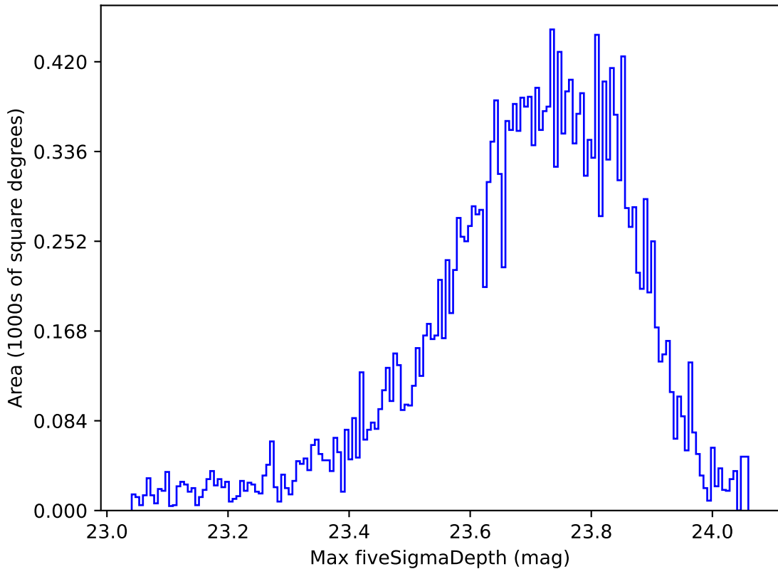
weather_cloudso14v3.4_10yrs All sky u band: Max fiveSigmaDepth
