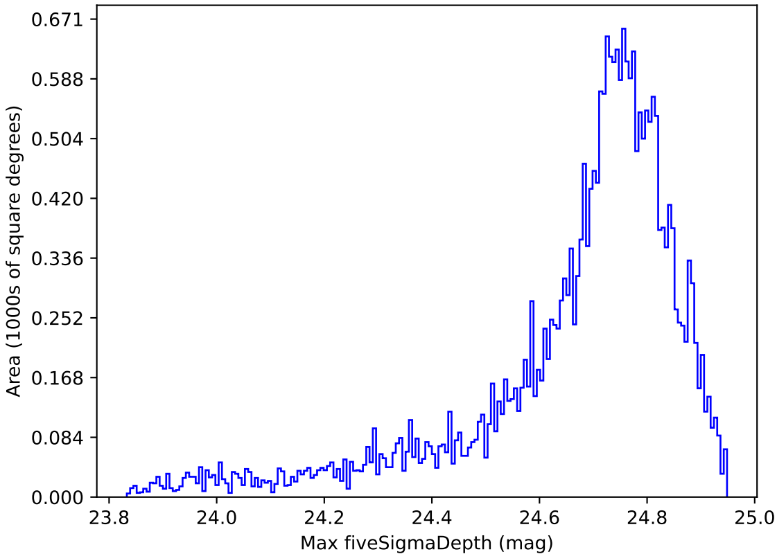
weather_cloudso14v3.4_10yrs All sky r band: Max fiveSigmaDepth
