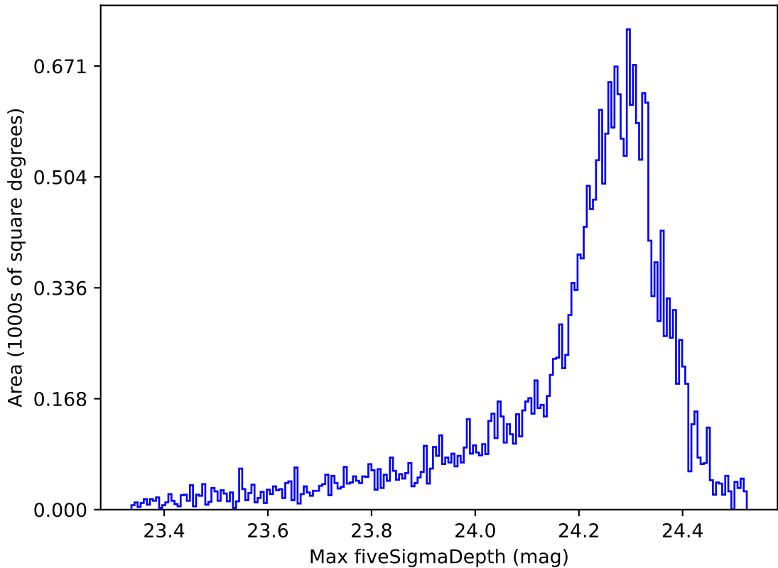
weather_cloudso14v3.4_10yrs All sky i band: Max fiveSigmaDepth
