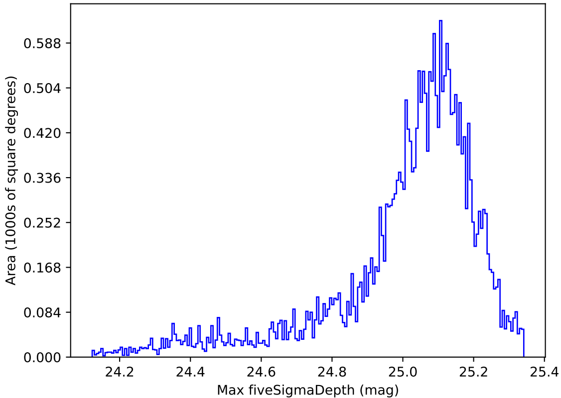
weather_cloudso14v3.4_10yrs All sky g band: Max fiveSigmaDepth
