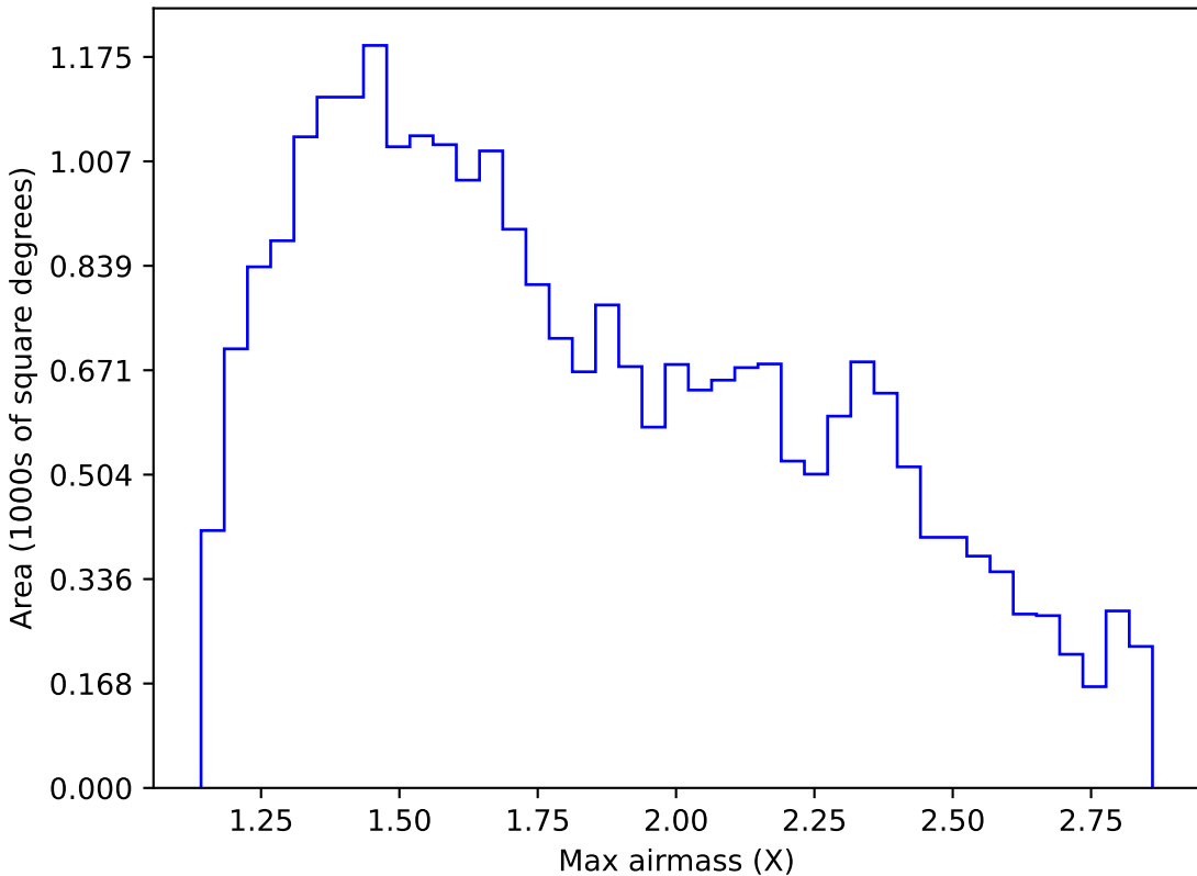
weather_cloudso14v3.4_10yrs Yr 1 z band: Max airmass
