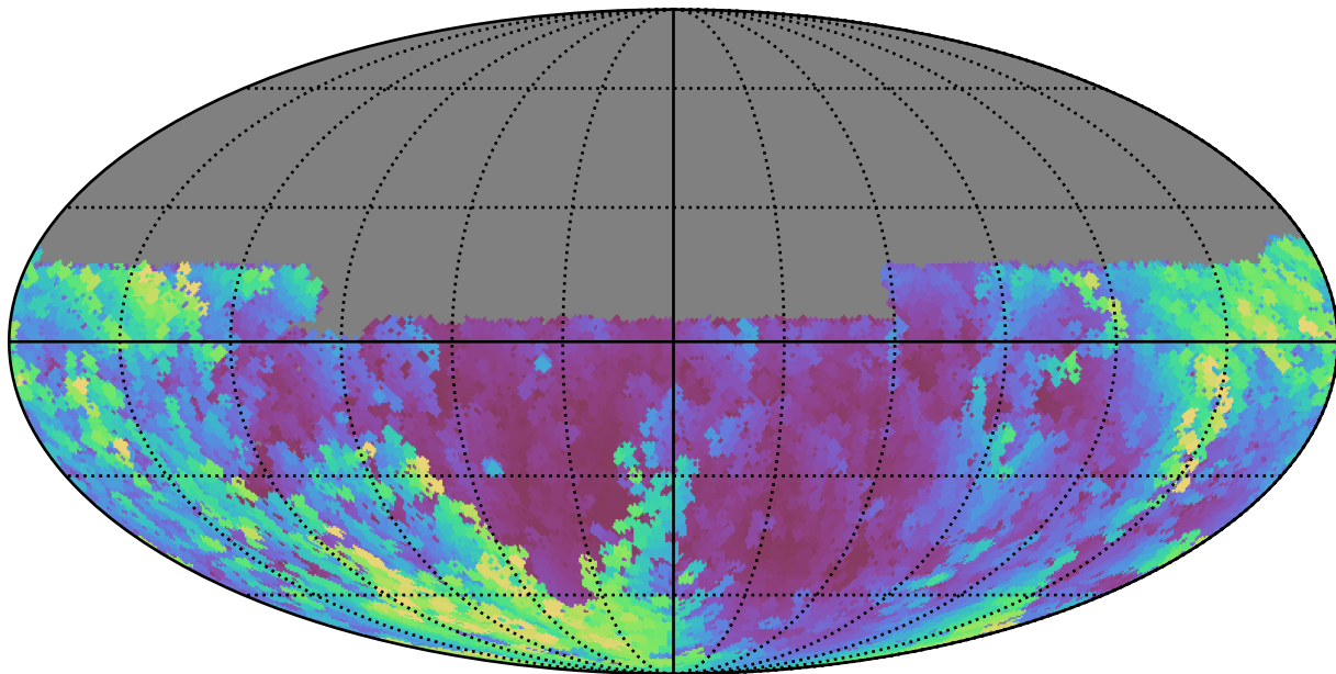
weather_cloudso14v3.4_10yrs Yr 1 y band: Max airmass
