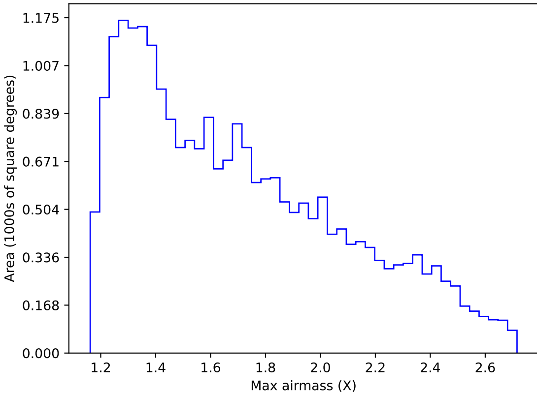
weather_cloudso14v3.4_10yrs Yr 1 y band: Max airmass
