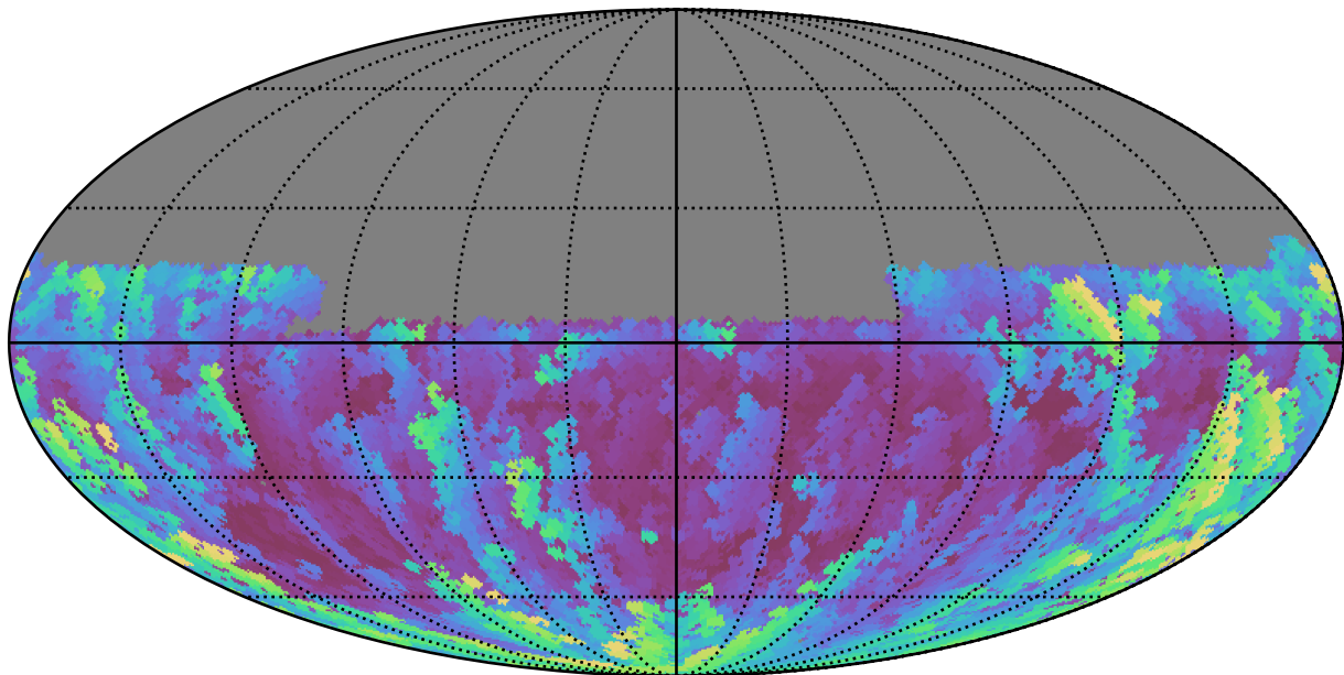
weather_cloudso14v3.4_10yrs Yr 1 u band: Max airmass
