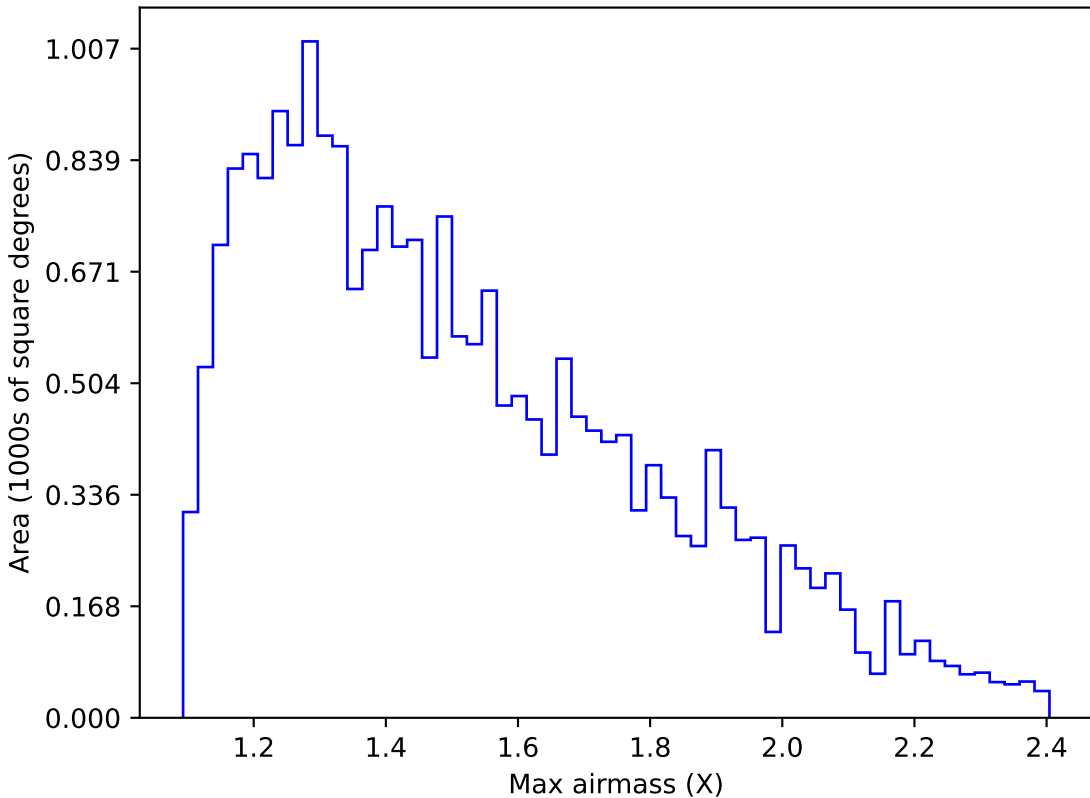
weather_cloudso14v3.4_10yrs Yr 1 u band: Max airmass
