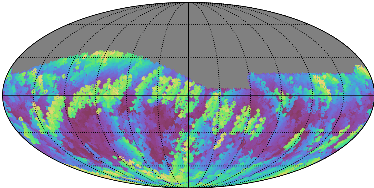
weather_cloudso14v3.4_10yrs Yr 1 r band: Max airmass
