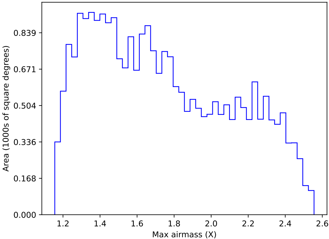
weather_cloudso14v3.4_10yrs Yr 1 r band: Max airmass
