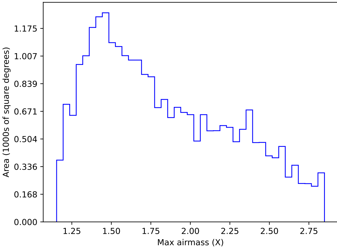
weather_cloudso14v3.4_10yrs Yr 1 i band: Max airmass
