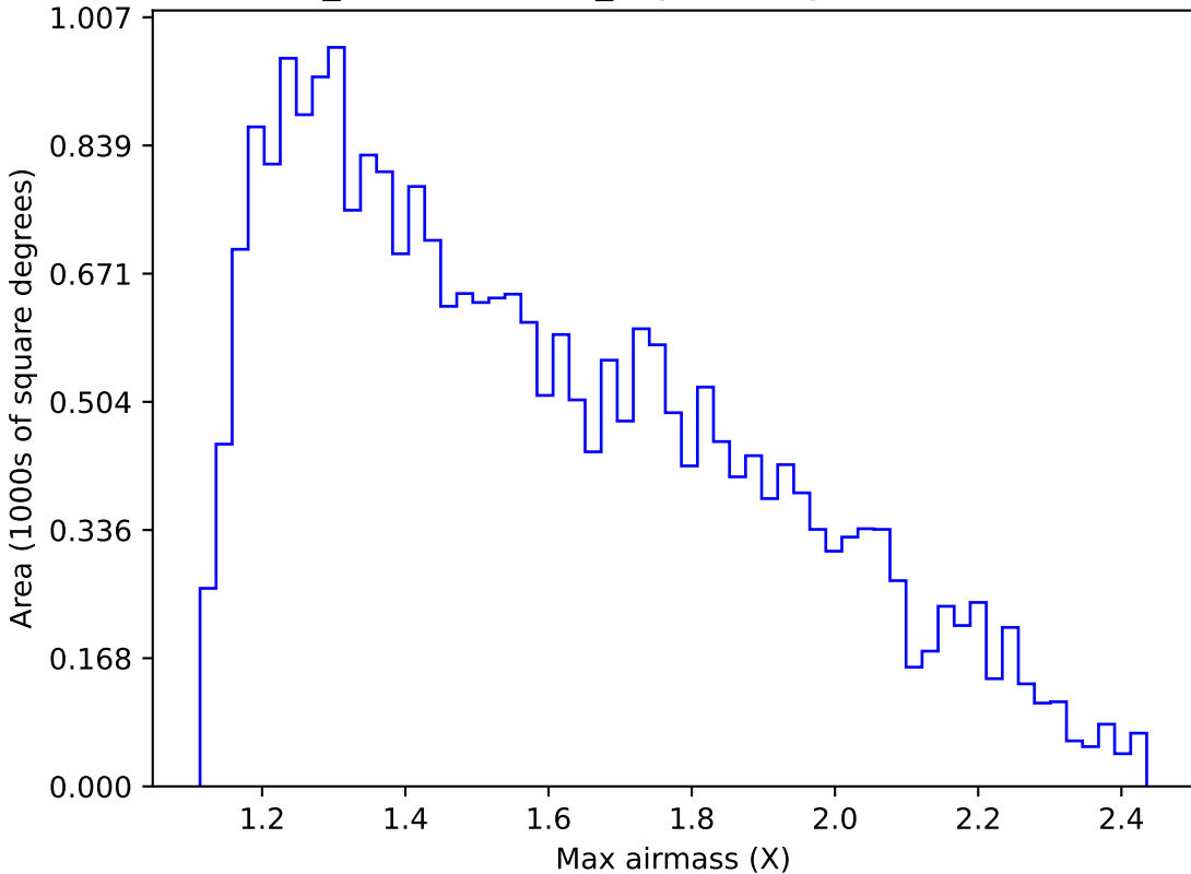
weather_cloudso14v3.4_10yrs Yr 1 g band: Max airmass
