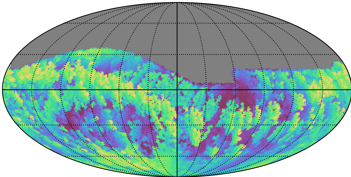
weather_cloudso14v3.4_10yrs Yr 1 all bands: Max airmass
