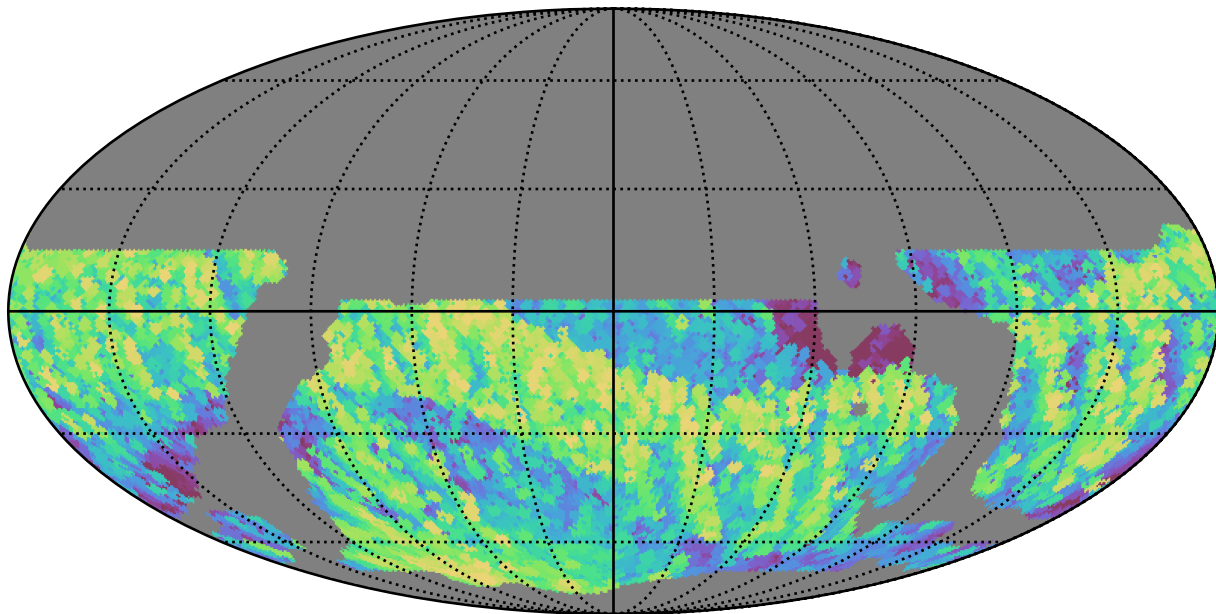
weather_cloudso14v3.4_10yrs WFD z band: Max airmass
