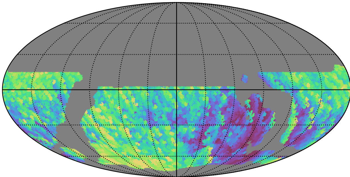
weather_cloudso14v3.4_10yrs WFD y band: Max airmass
