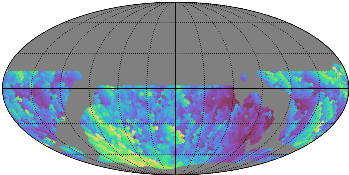
weather_cloudso14v3.4_10yrs WFD u band: Max airmass
