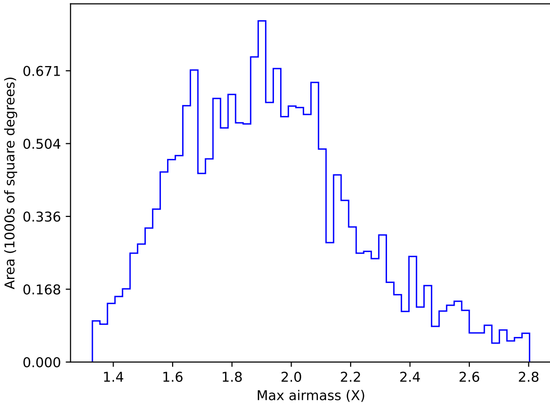
weather_cloudso14v3.4_10yrs WFD u band: Max airmass
