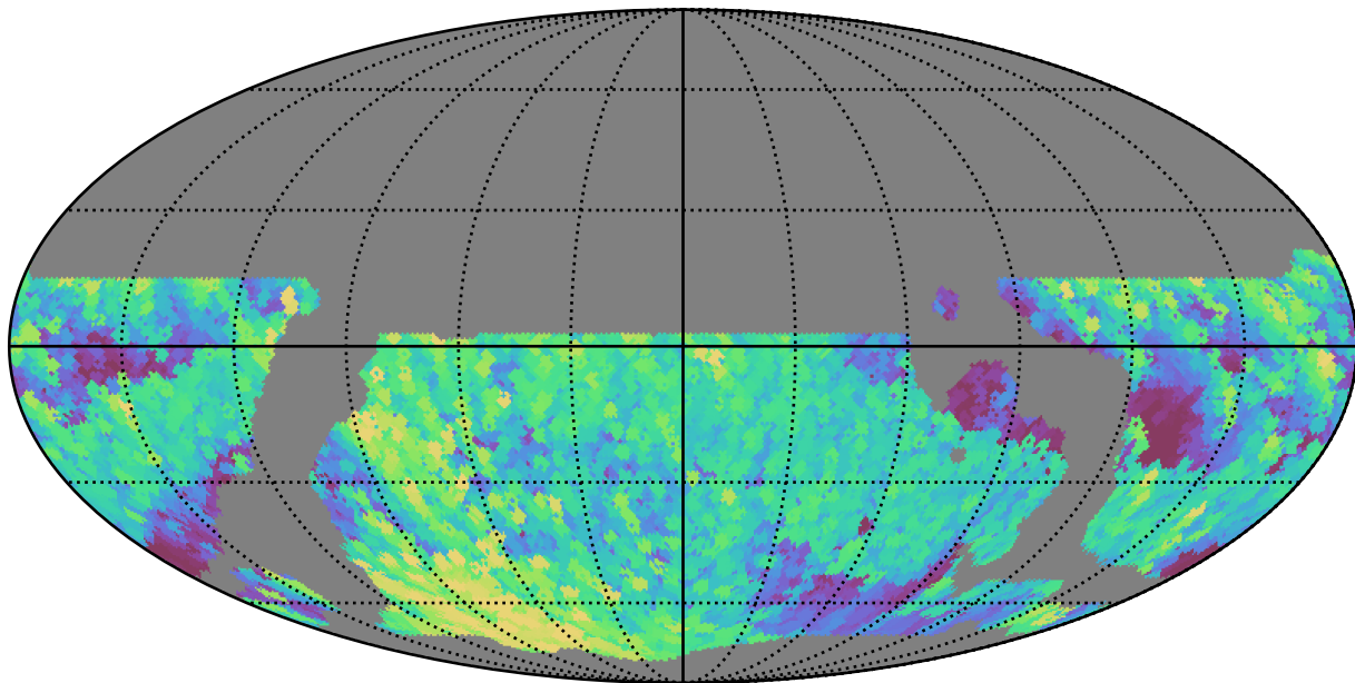
weather_cloudso14v3.4_10yrs WFD r band: Max airmass
