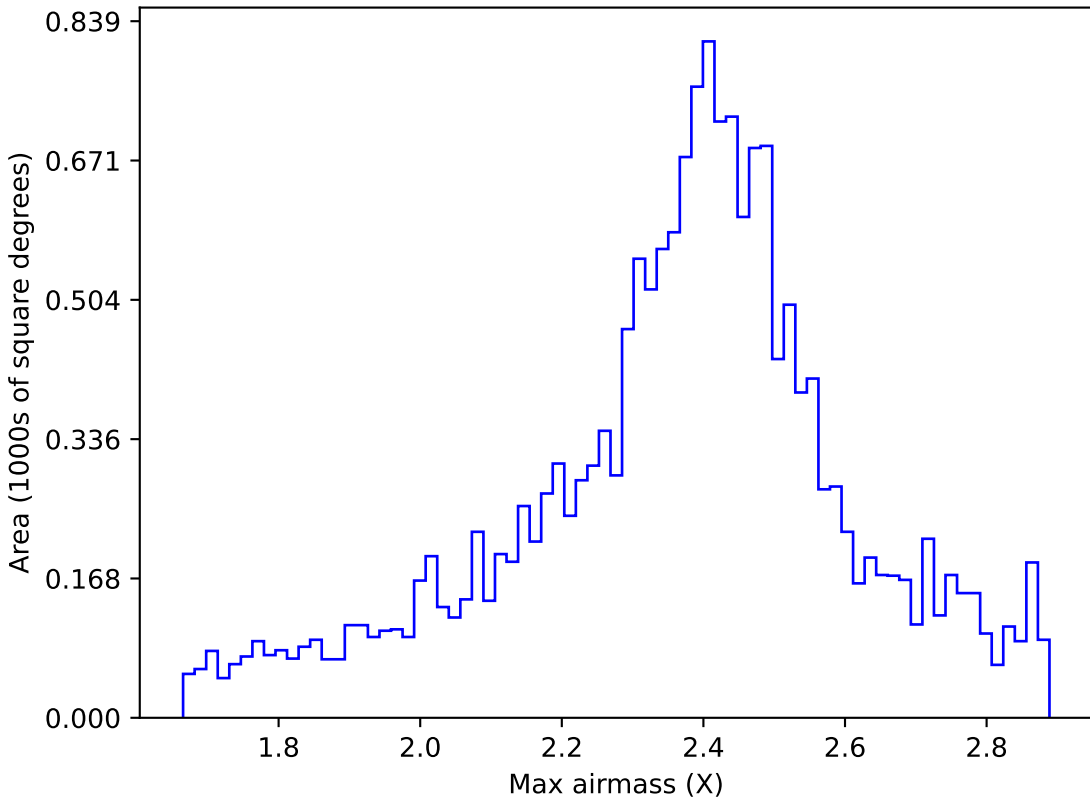
weather_cloudso14v3.4_10yrs WFD r band: Max airmass
