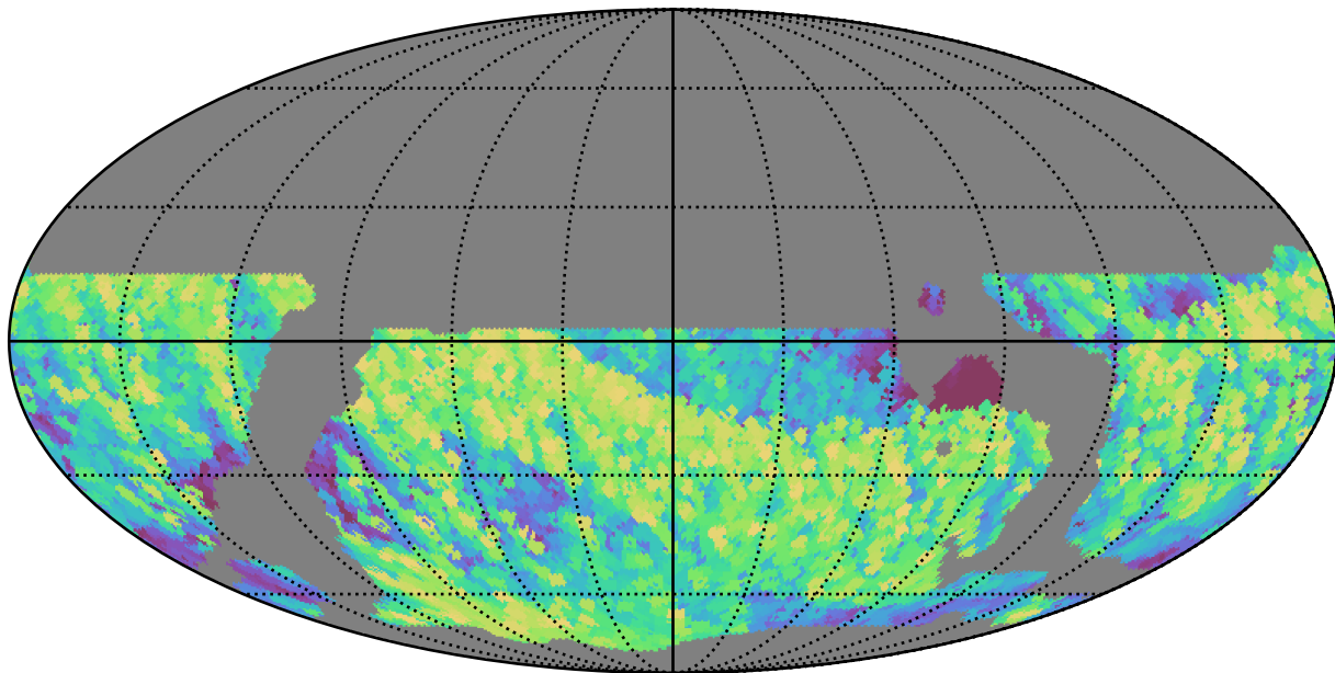
weather_cloudso14v3.4_10yrs WFD i band: Max airmass
