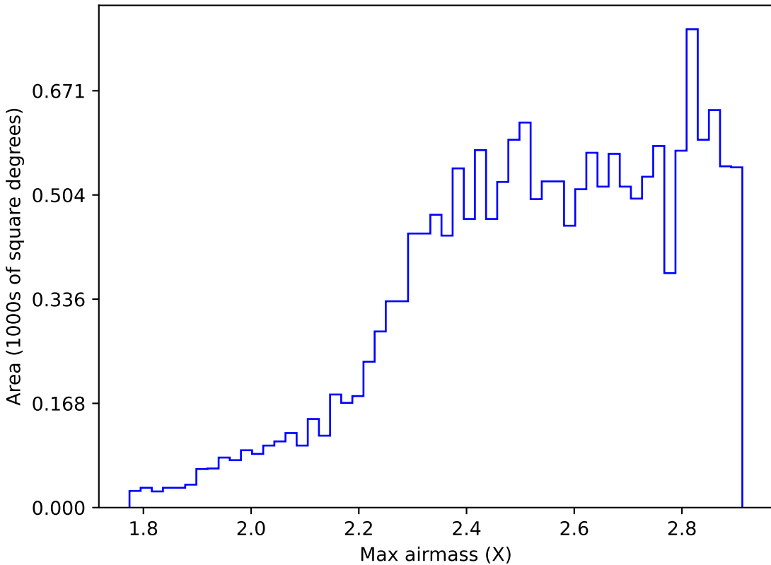
weather_cloudso14v3.4_10yrs WFD i band: Max airmass
