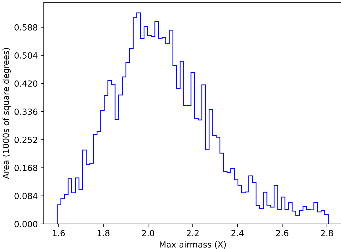
weather_cloudso14v3.4_10yrs WFD g band: Max airmass
