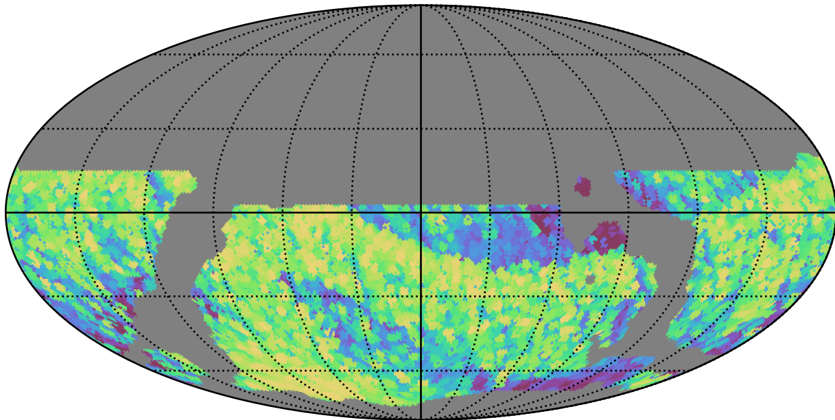
weather_cloudso14v3.4_10yrs WFD all bands: Max airmass
