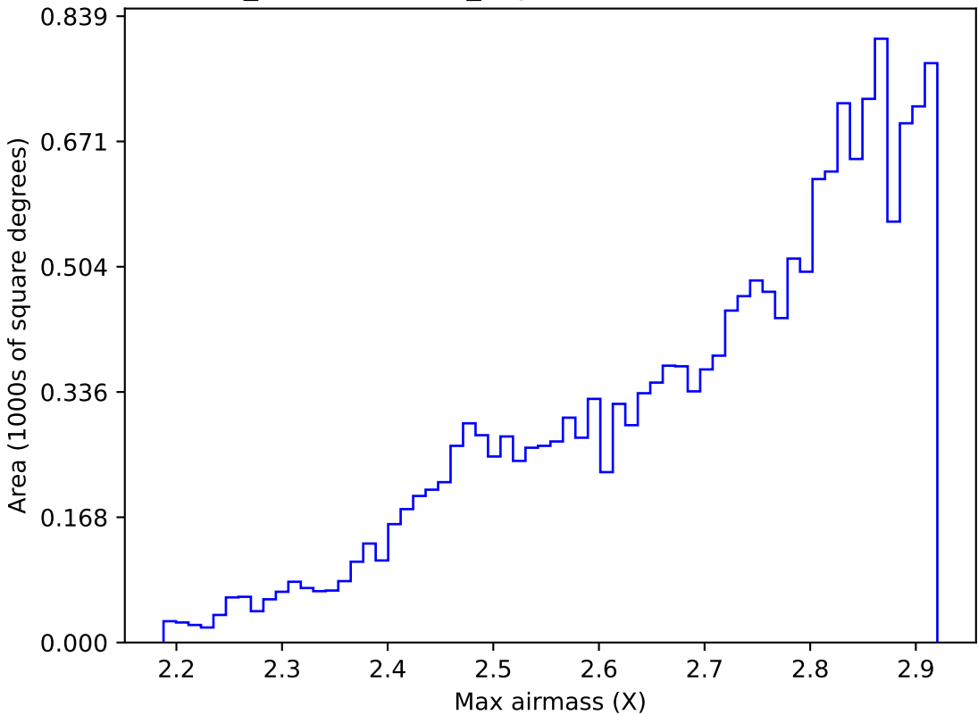
weather_cloudso14v3.4_10yrs WFD all bands: Max airmass
