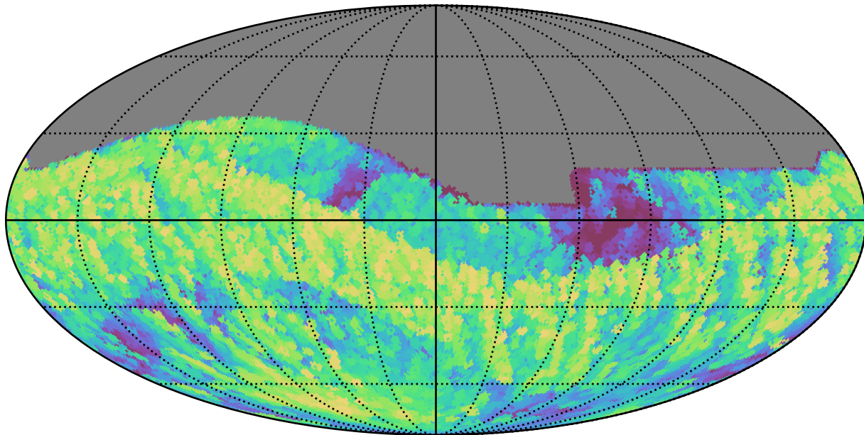
weather_cloudso14v3.4_10yrs All sky z band: Max airmass
