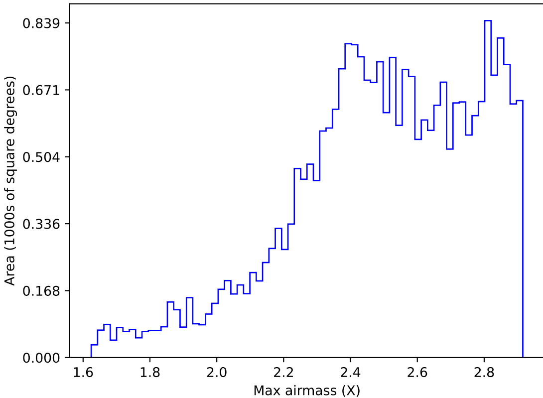
weather_cloudso14v3.4_10yrs All sky z band: Max airmass
