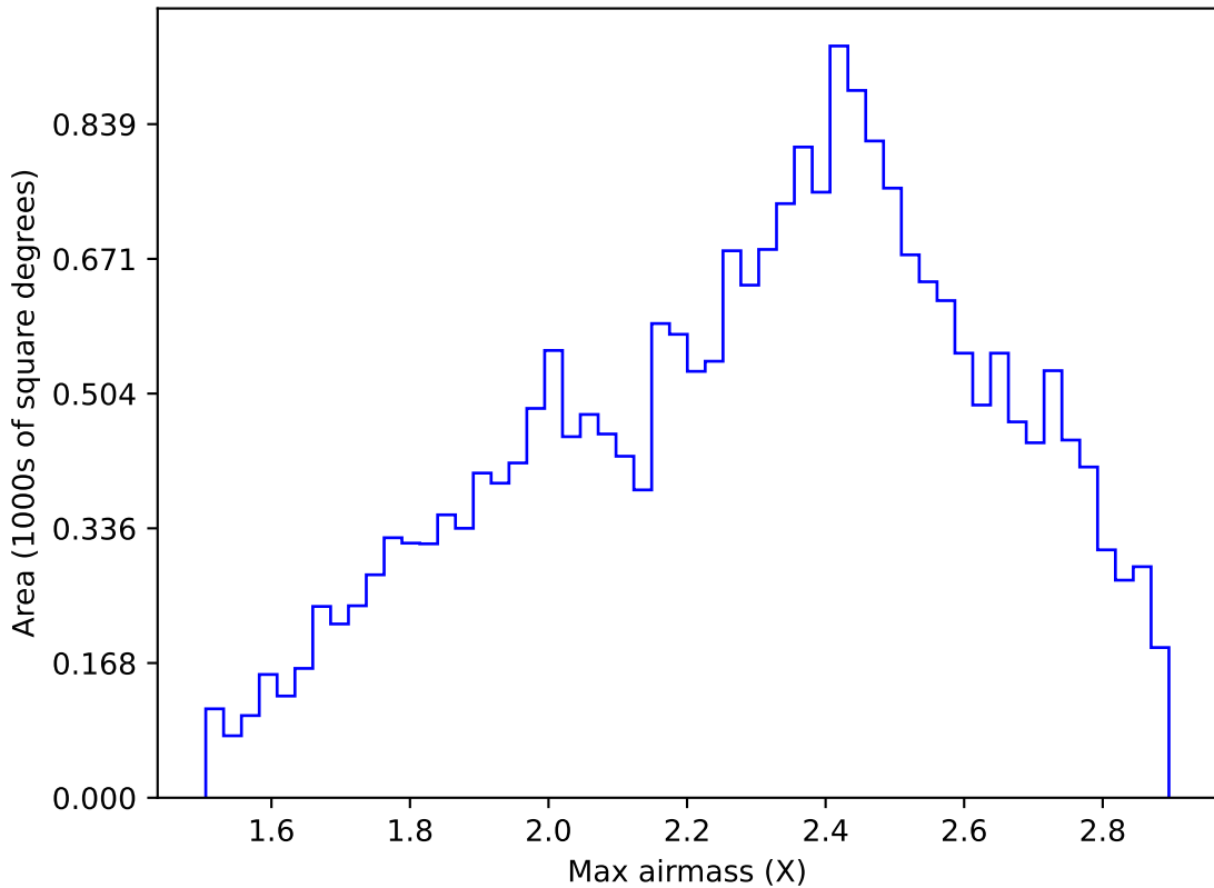
weather_cloudso14v3.4_10yrs All sky y band: Max airmass
