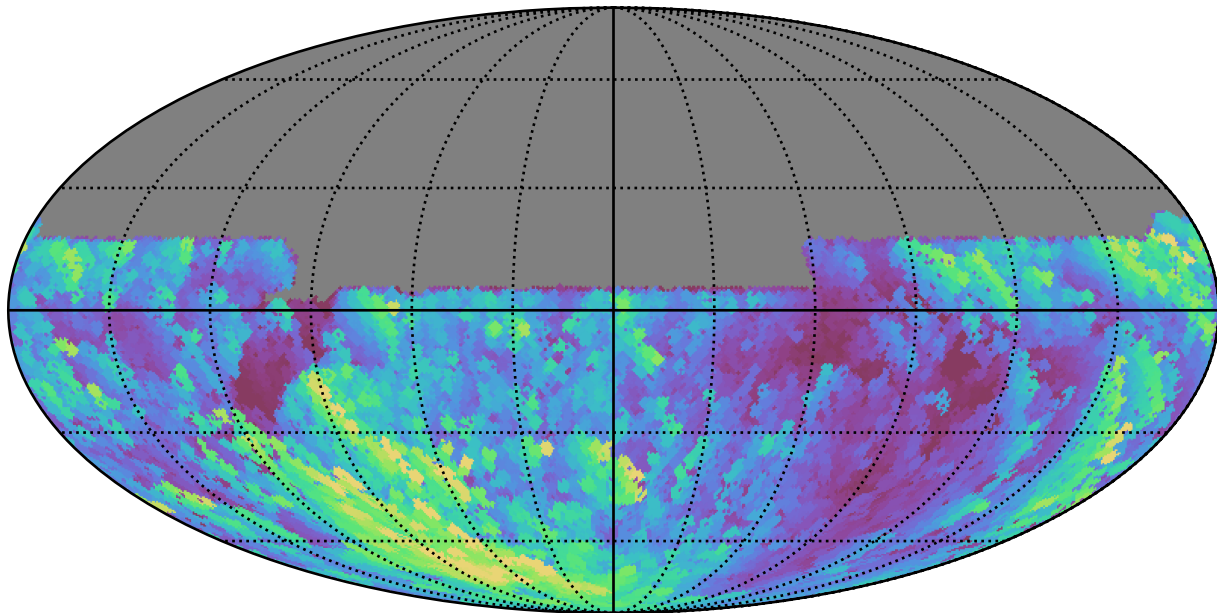
weather_cloudso14v3.4_10yrs All sky u band: Max airmass
