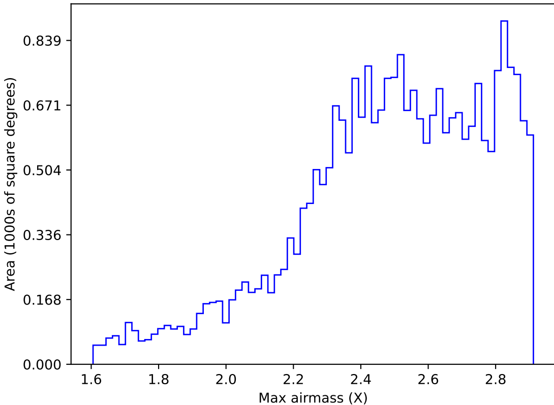
weather_cloudso14v3.4_10yrs All sky i band: Max airmass
