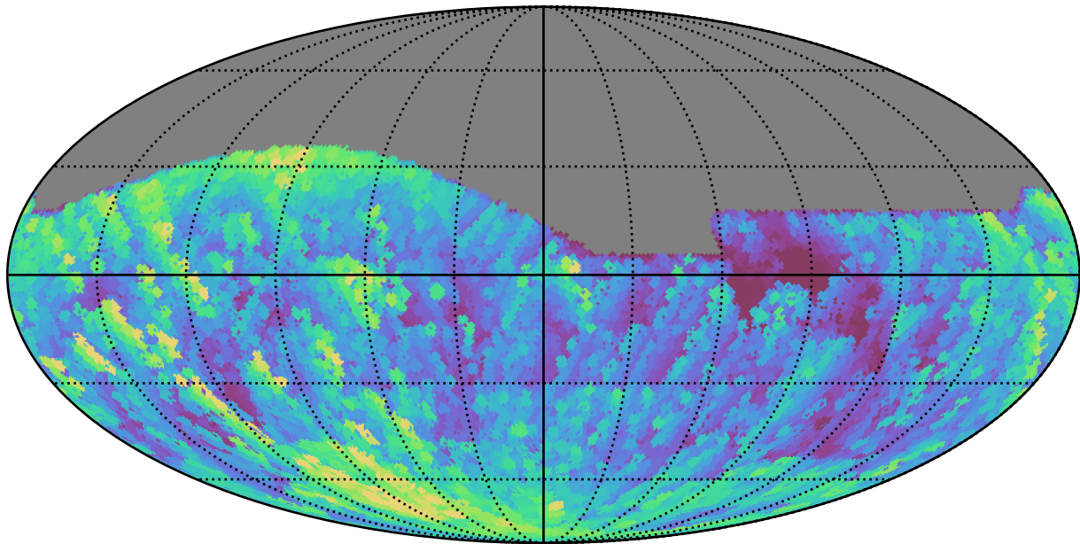
weather_cloudso14v3.4_10yrs All sky g band: Max airmass
