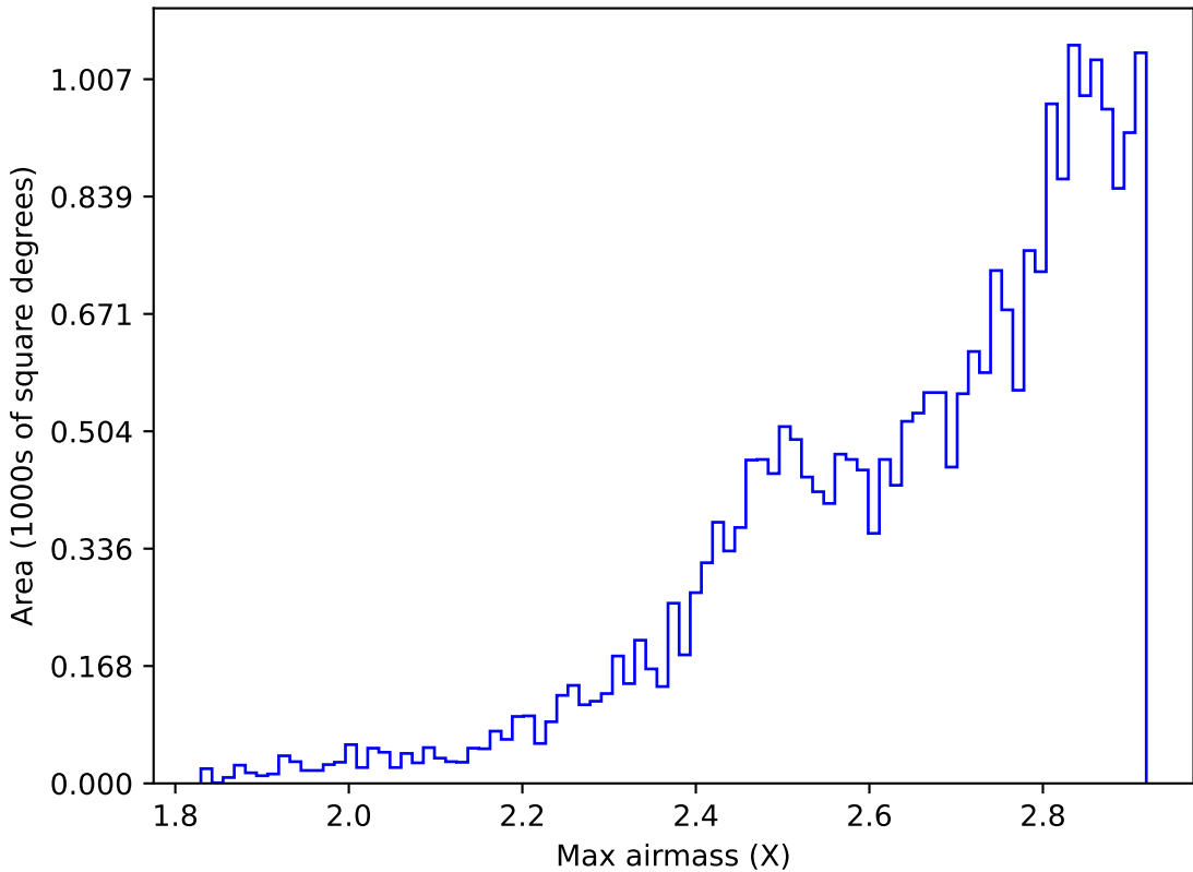
weather_cloudso14v3.4_10yrs All sky all bands: Max airmass
