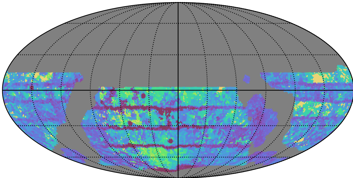
weather_cloudso14v3.4_10yrs WFD z band: Max Inter-Night Gap
