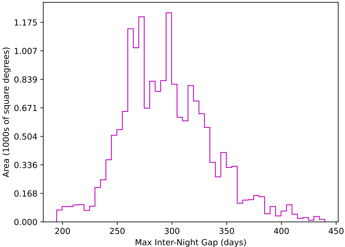
weather_cloudso14v3.4_10yrs WFD z band: Max Inter-Night Gap
