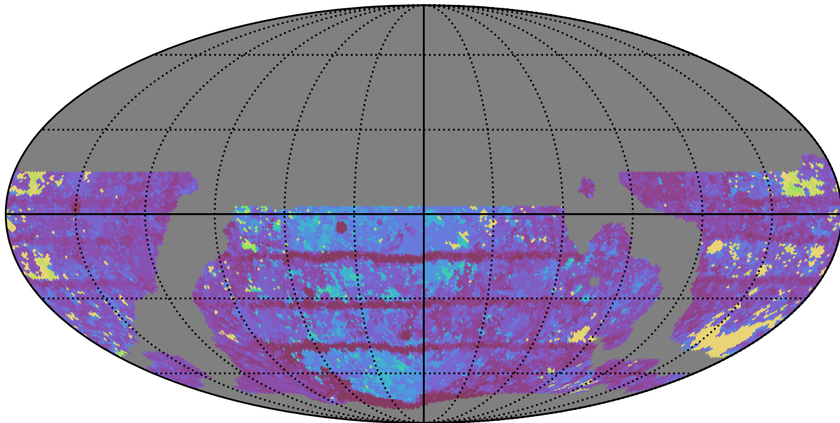
weather_cloudso14v3.4_10yrs WFD y band: Max Inter-Night Gap
