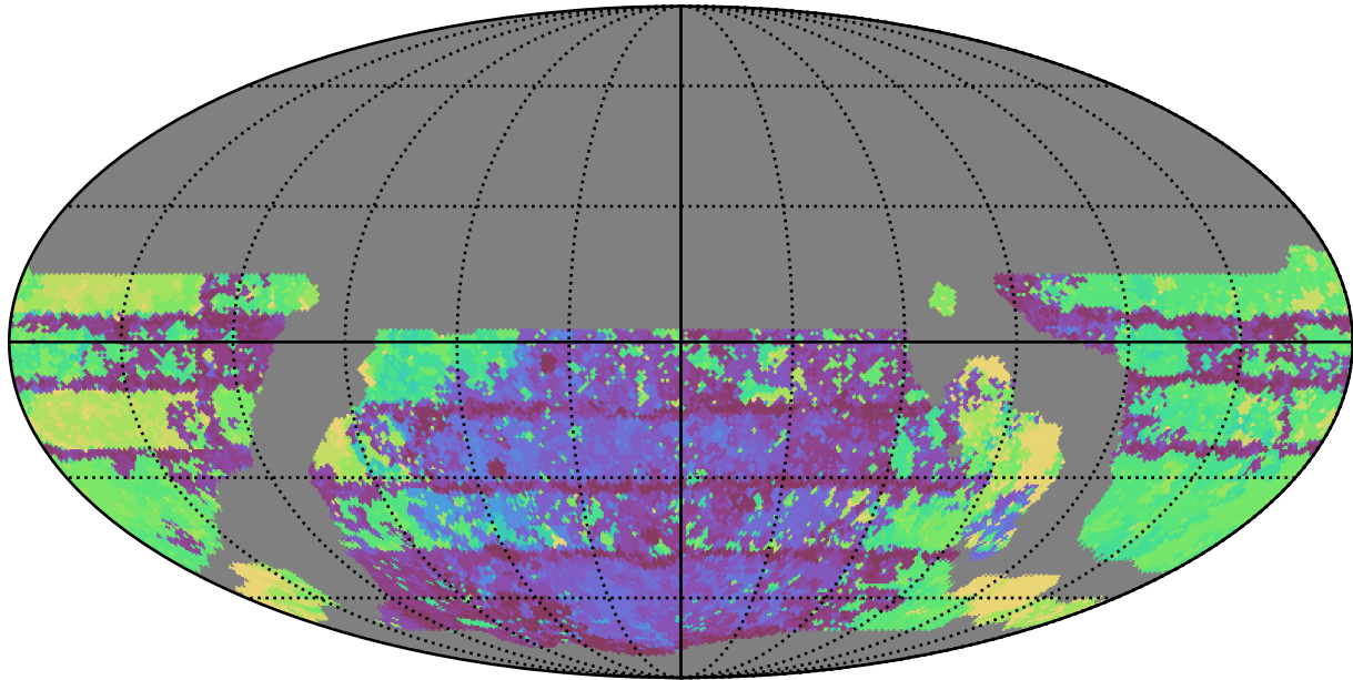
weather_cloudso14v3.4_10yrs WFD u band: Max Inter-Night Gap
