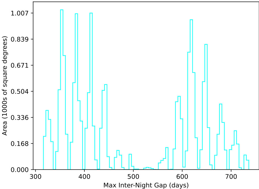
weather_cloudso14v3.4_10yrs WFD u band: Max Inter-Night Gap
