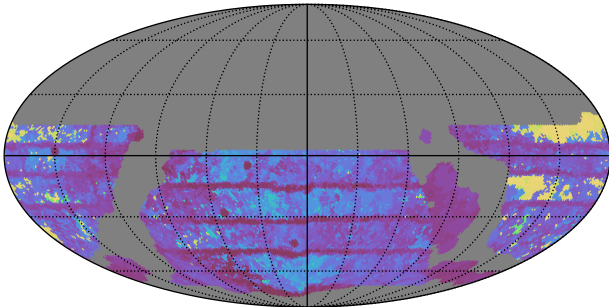
weather_cloudso14v3.4_10yrs WFD r band: Max Inter-Night Gap
