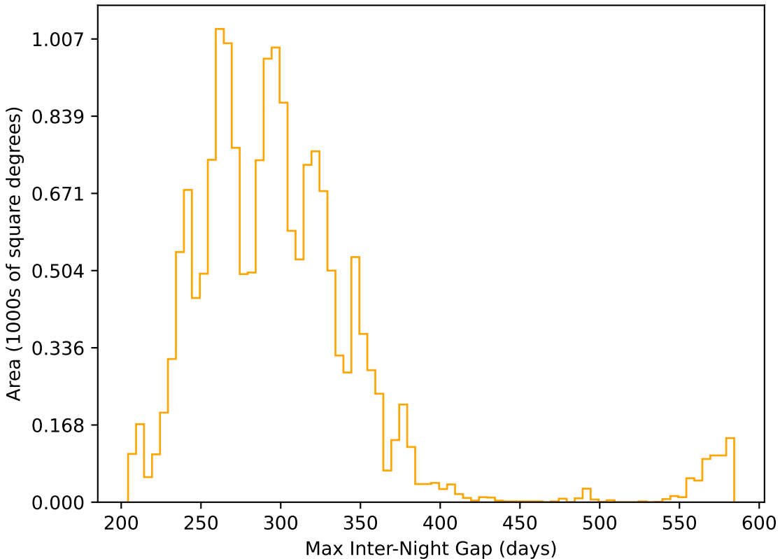
weather_cloudso14v3.4_10yrs WFD r band: Max Inter-Night Gap
