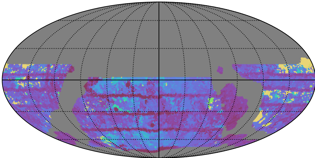
weather_cloudso14v3.4_10yrs WFD i band: Max Inter-Night Gap
